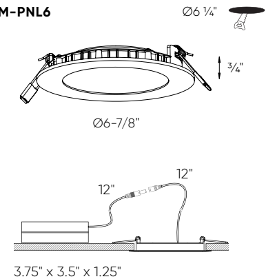
SM-PNL6 Ø6 1/4"
